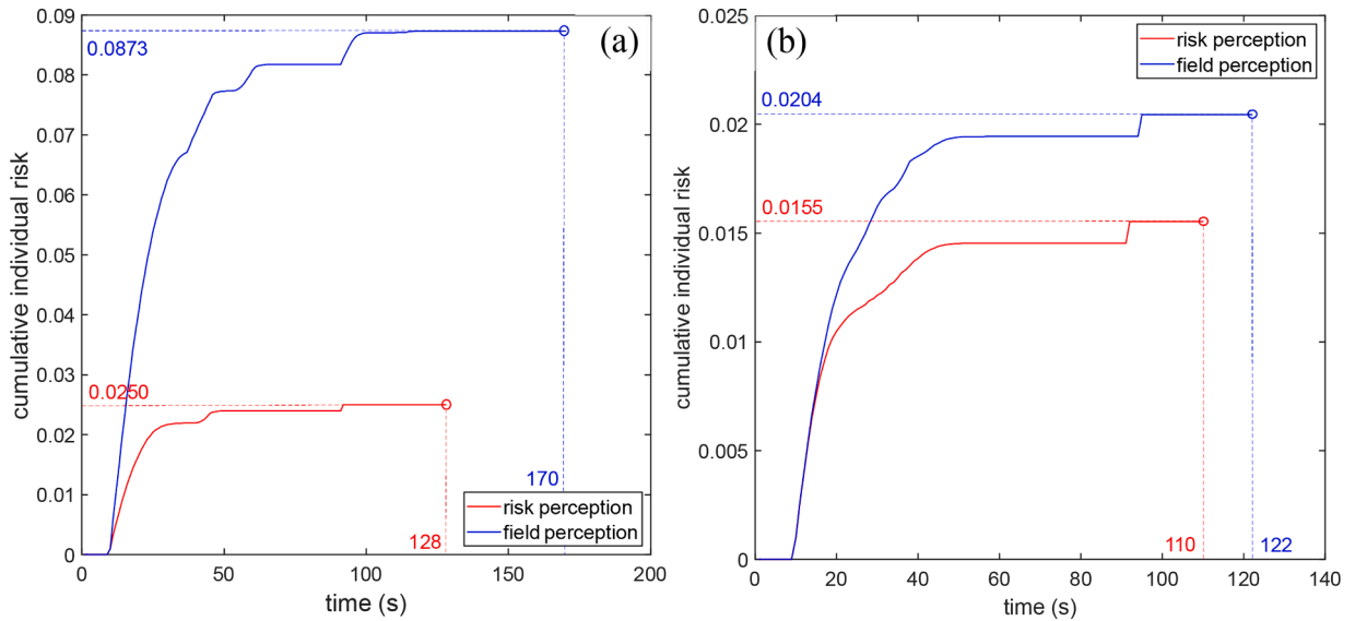
Fig. 9. The CIR-time curves of the evacuation paths planned by the field-perception and pre-perception algorithm and the field-perception-only algorithm. (a) without designated exits, (b) with the three designated exits.
